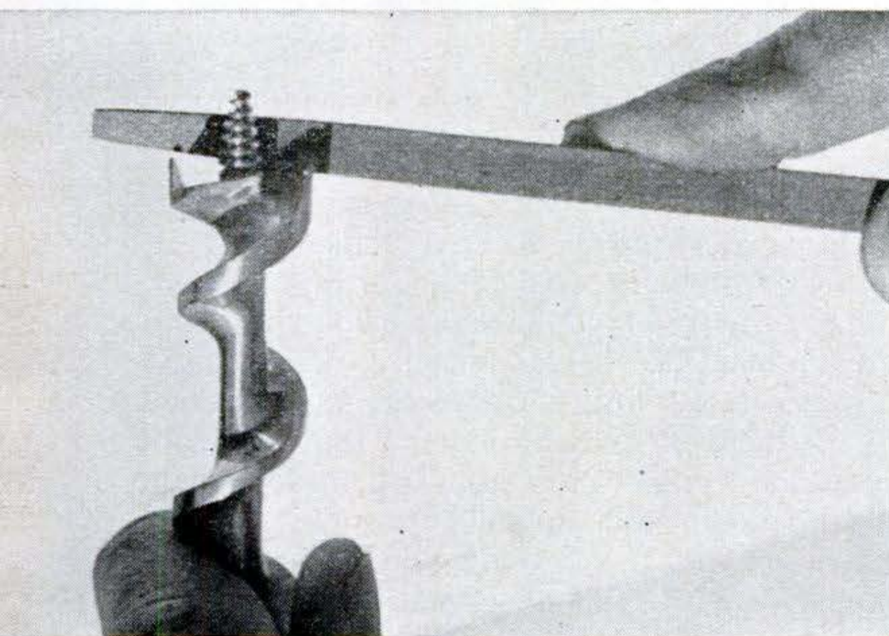
ONE-HAND GRIP , with first finger extended for control, is best for sharpening tools not held in a vise. Choice for this job is auger-bit file made for the purpose.
